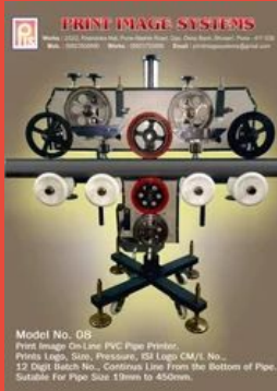
On-Line Rigid PVC Pipe Printer
