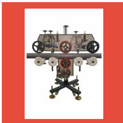
On-Line PVC Pipe Printing Machine
